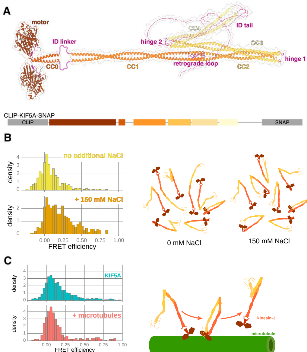
Figure 3 - Investigating the dynamic heterogeneity of Kinesin-1
