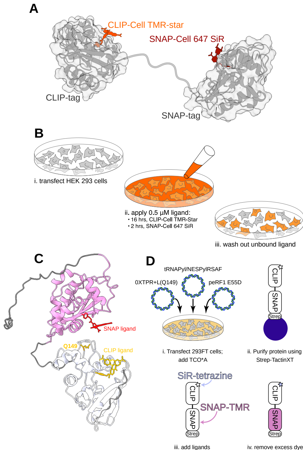
Figure 2 - In-cell labelling for smFRET using self-labelling enzymes
